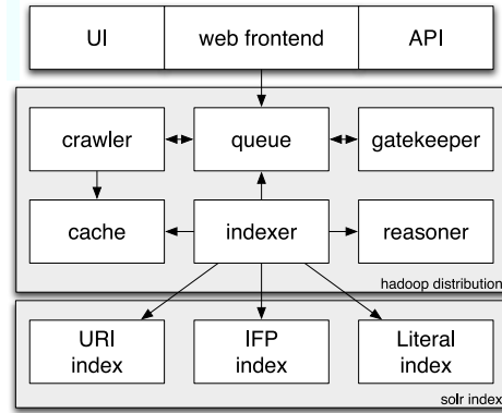
Fig. 4. Sindice architecture
